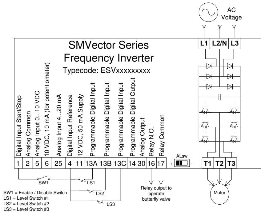
Figure 2: SMVector Wiring Diagram
