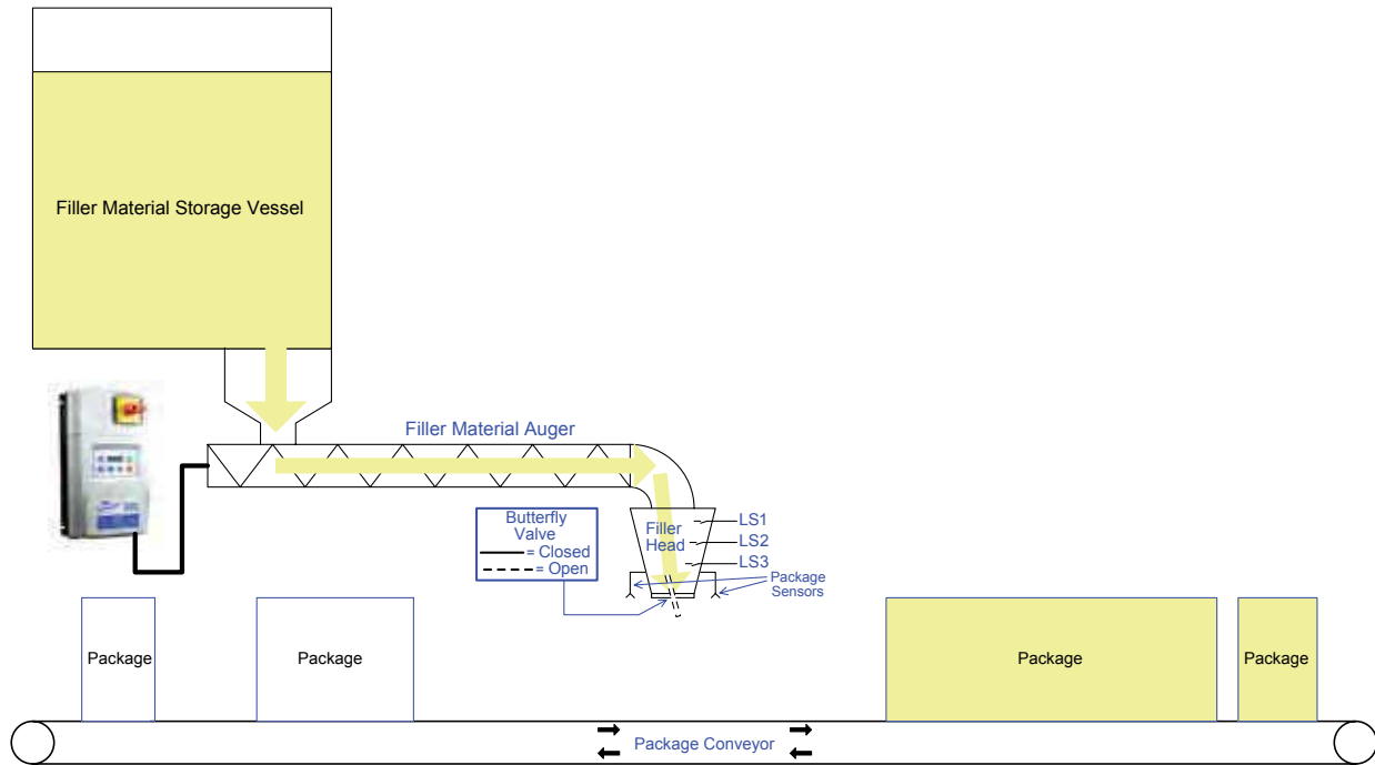
Figure 1: Package Filler Block Diagram
