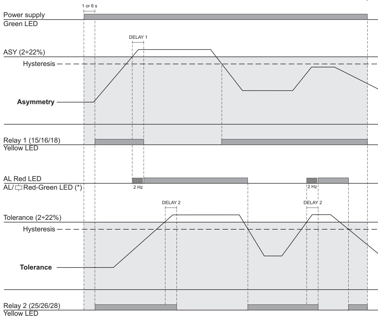
Fig. 14 Asymmetry and tolerance monitoring (2 x SPDT relay)
